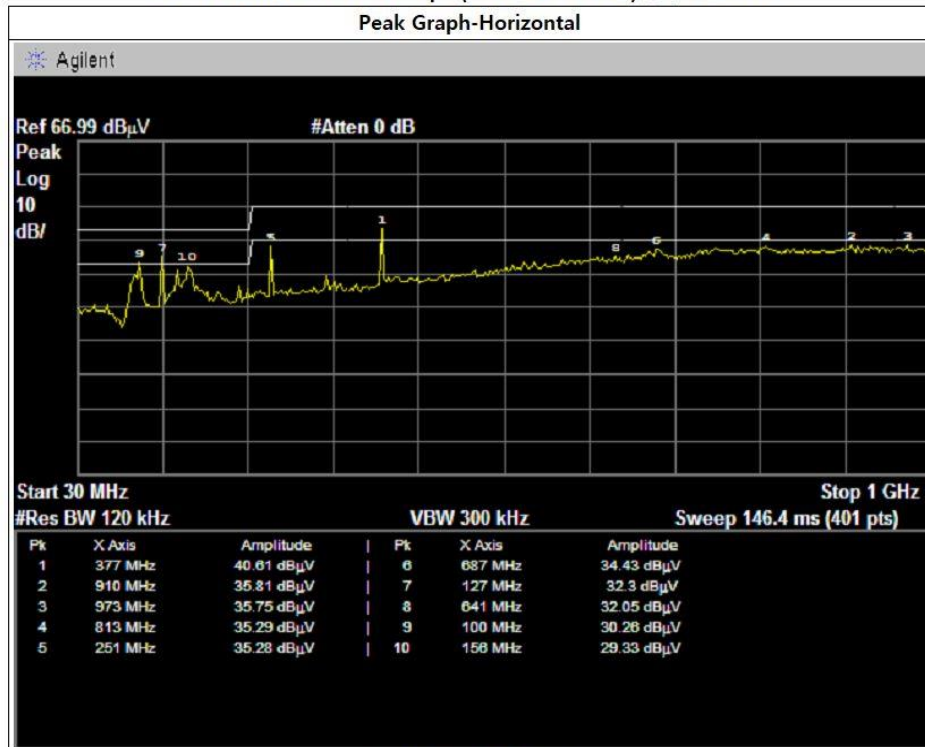
Radiated Emission Data Graph ( 30 MHz ~ 1 GHz ) 동작 2024.08.23
